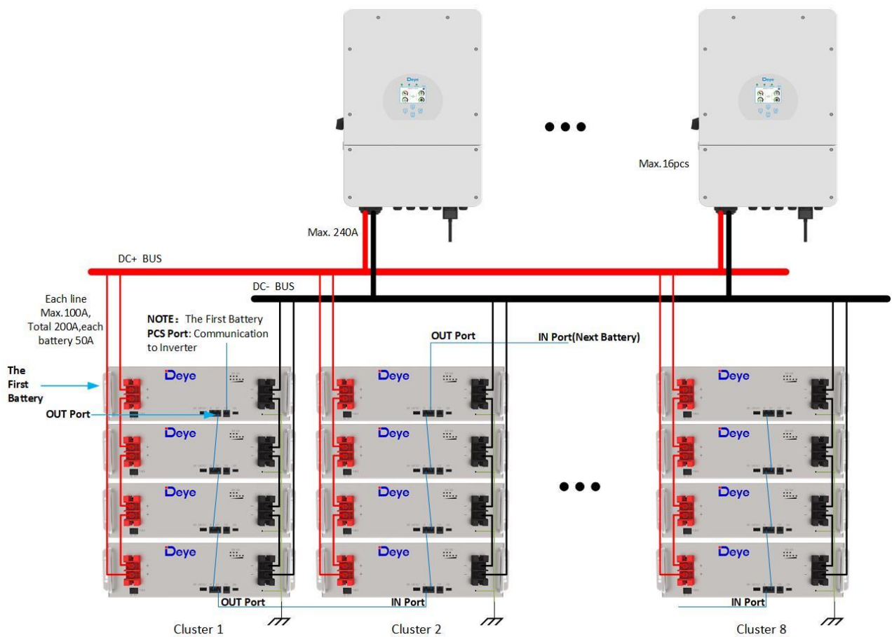
Figure 5-4: Multiple Batteries Connections
