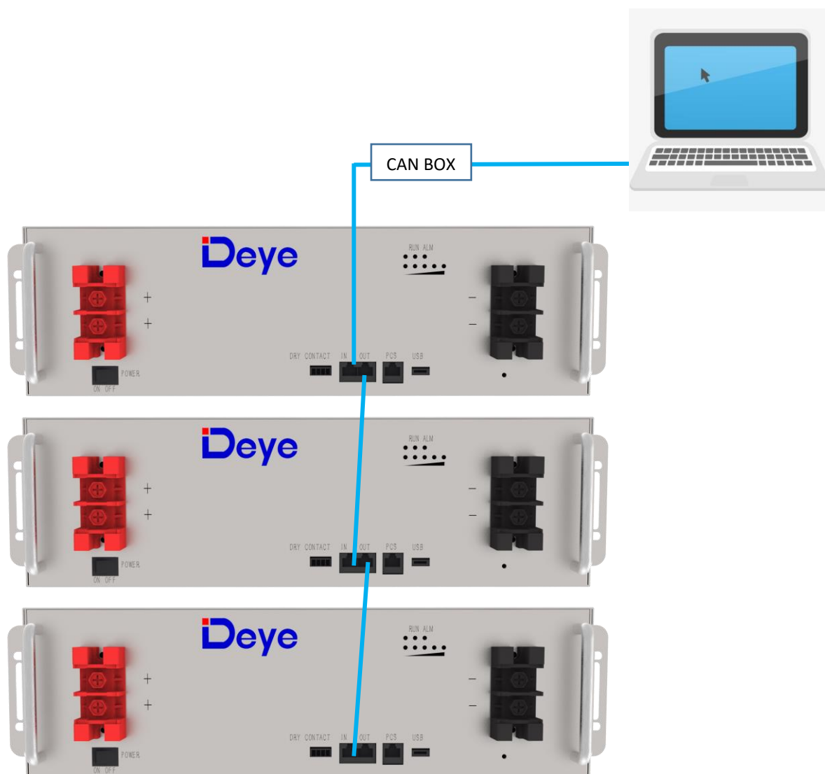
Figure 5-3: Communication Cable Connections between Battery and Computer
