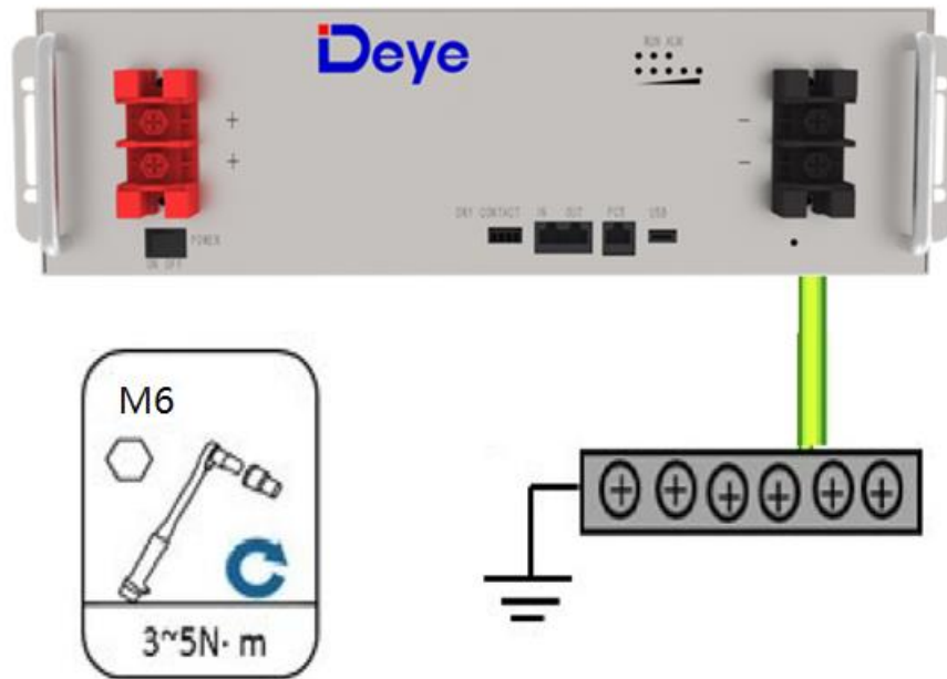
Figure 5-1: Install the Grounding Wire
