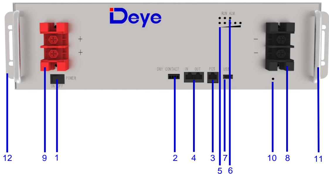
Figure 2-1: Front Panel Function Introduction
